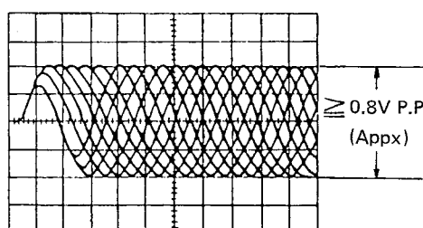
Fig. 2-1-3 RF Waveform
