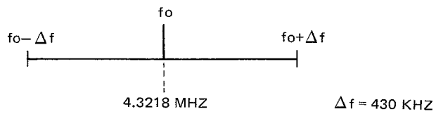
Fig. 2-7-1 PLL operating range
