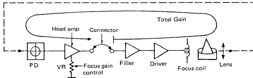
Fig. 2-2-1 Focus Servo Loop
