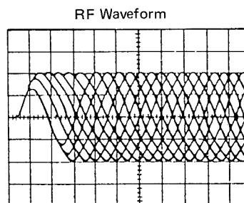
Waveform of optimum alignment
