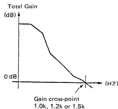
Fig. 2-3-2 Tracking servo characteristics
