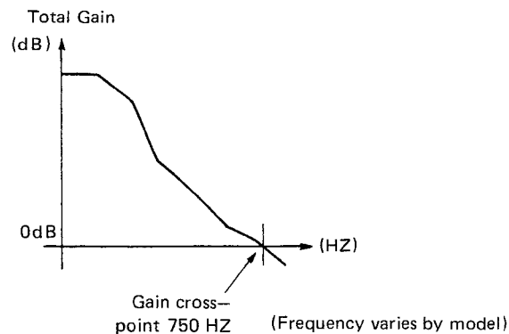
Fig. 2-2-2 Focus servo gain characteristics
