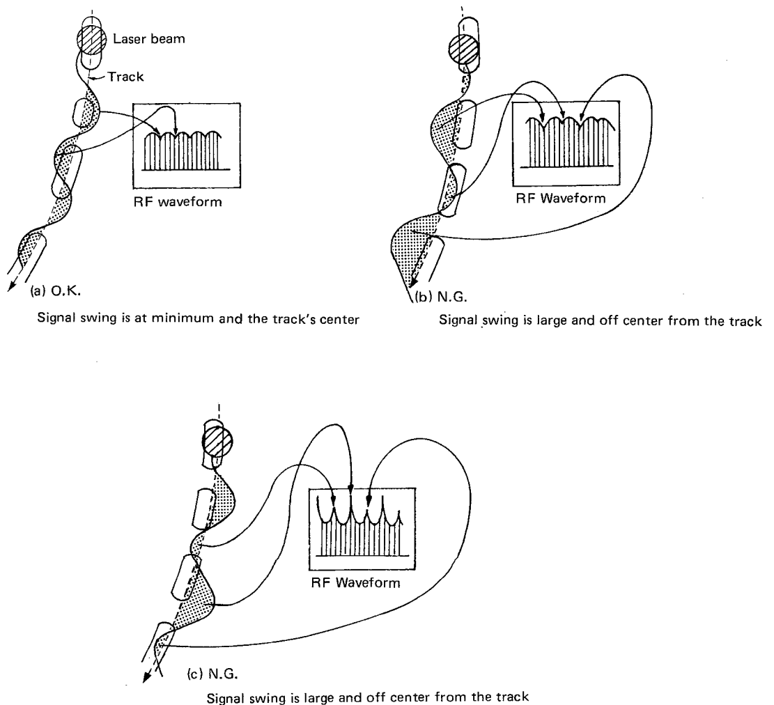
Fig. 2-6-1 Beam movement with error signal
